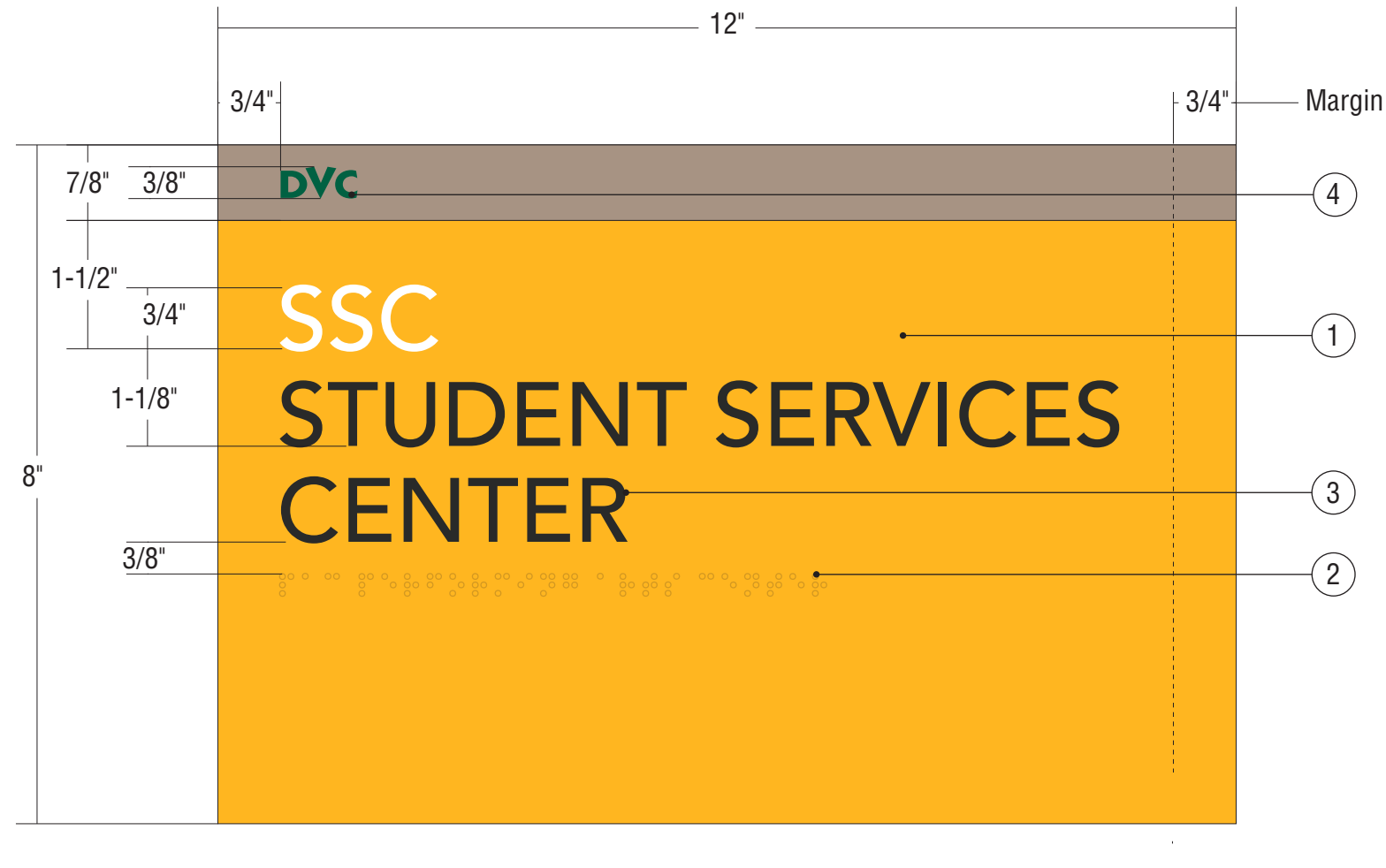
① FRONT VIEW Scale: 1/2 Size
