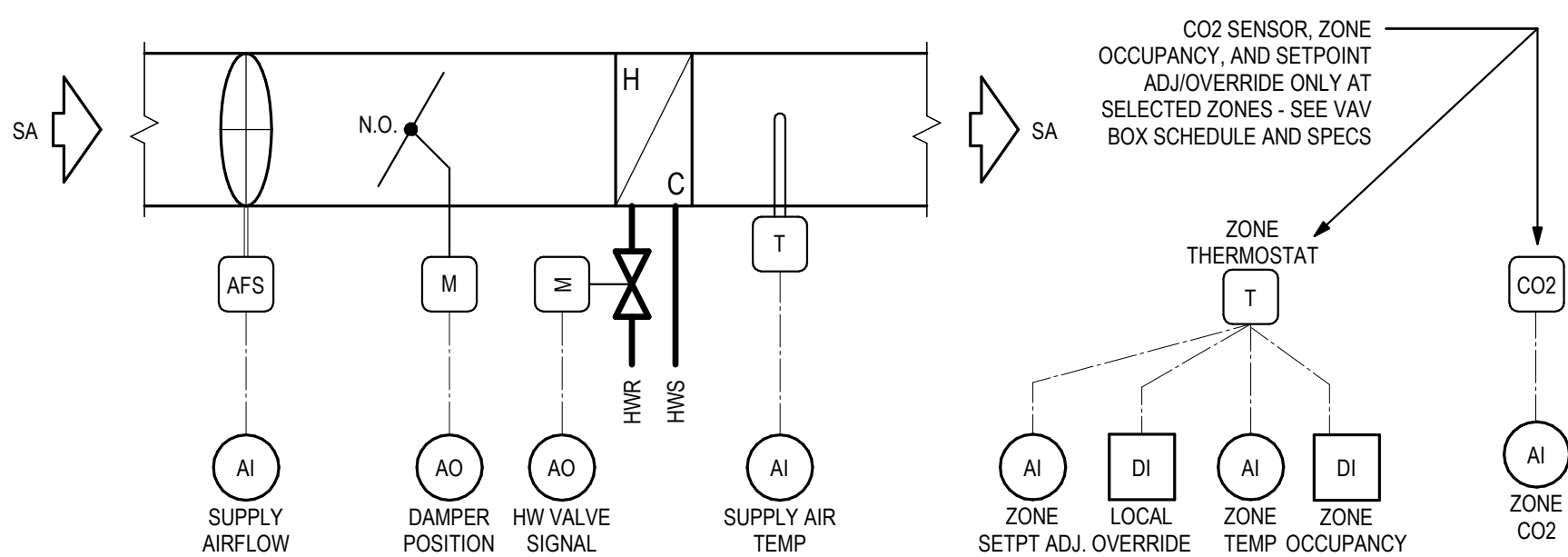
3 VAV REHEAT ZONE - EXISTING DDC AND PNEUMATIC
