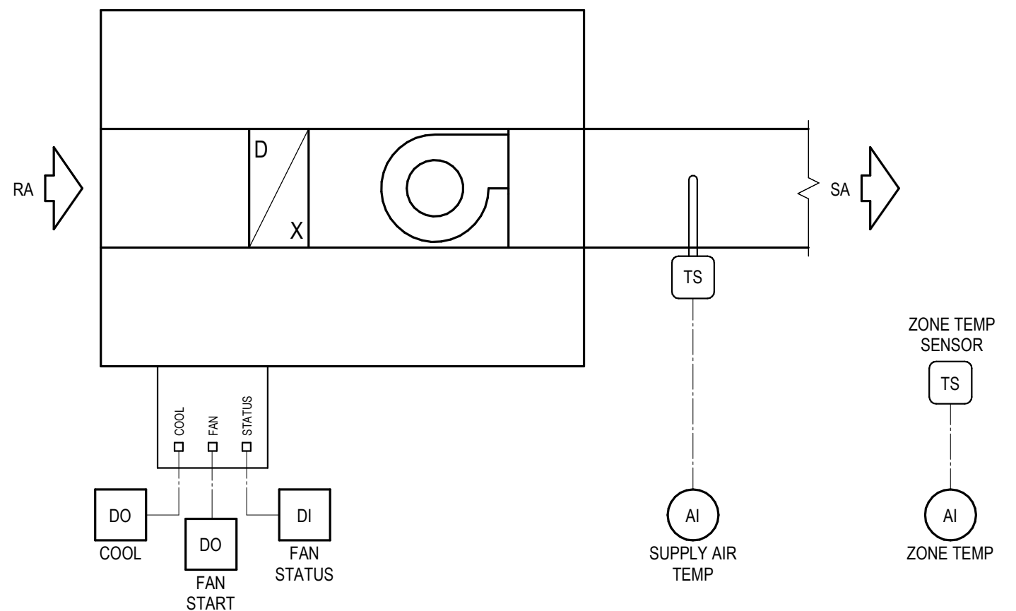
2 PACKAGED AC UNIT OR HEAT PUMP
