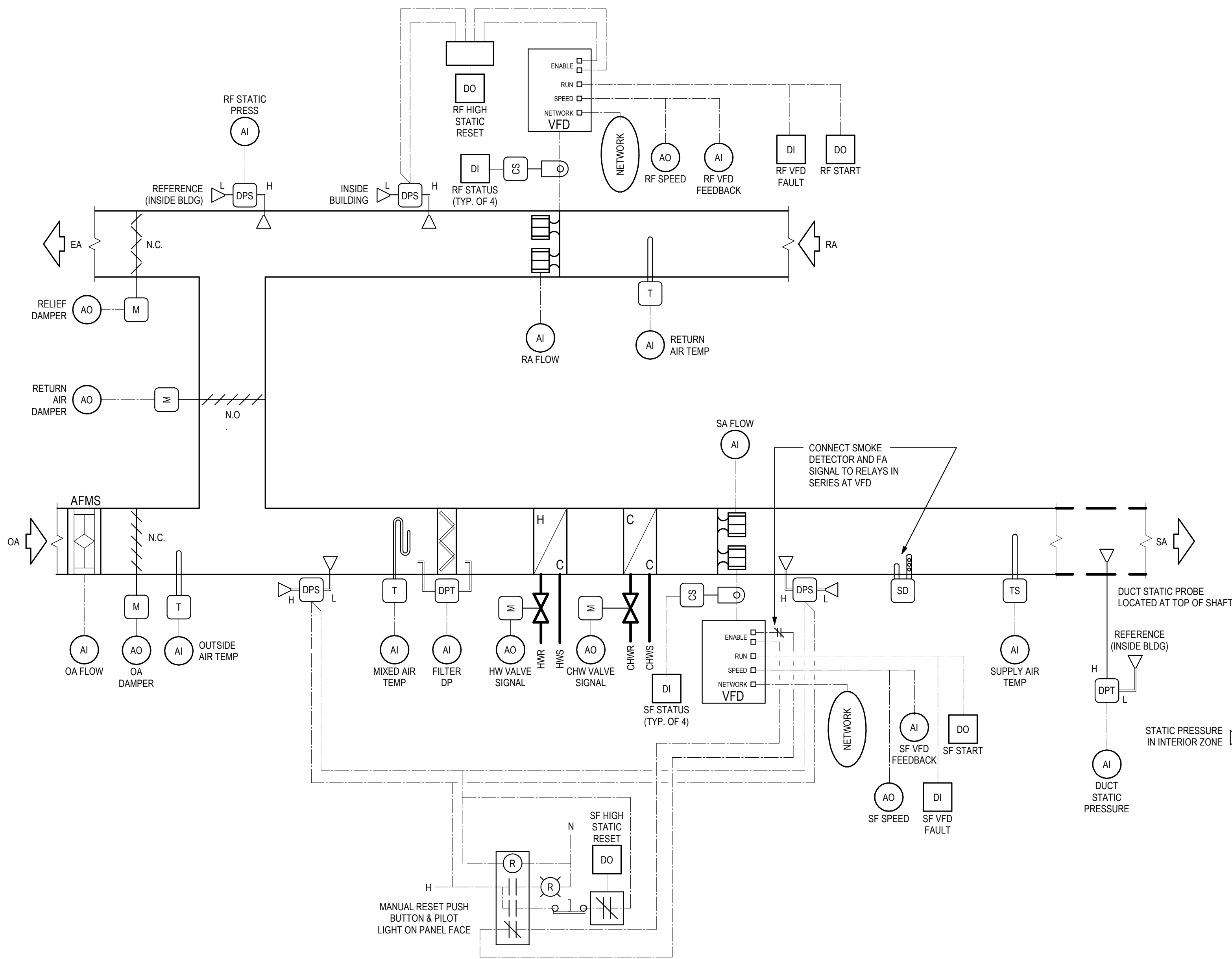
1 VAV AIR HANDLER WITH RETURN FAN AND HW/CHW COILS
